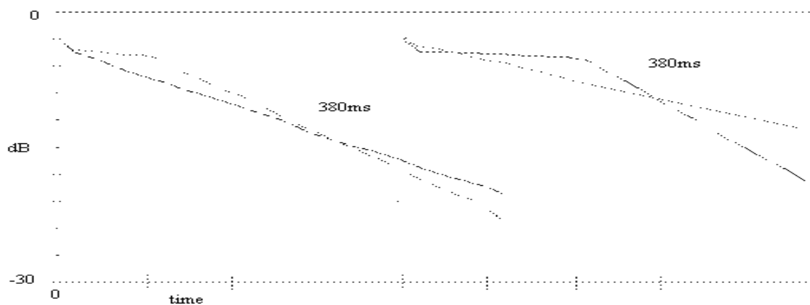
Figure 2: Two pairs of equally loud reverberation profiles - Schroeder integrals cross at ~380ms but not at -10dB
